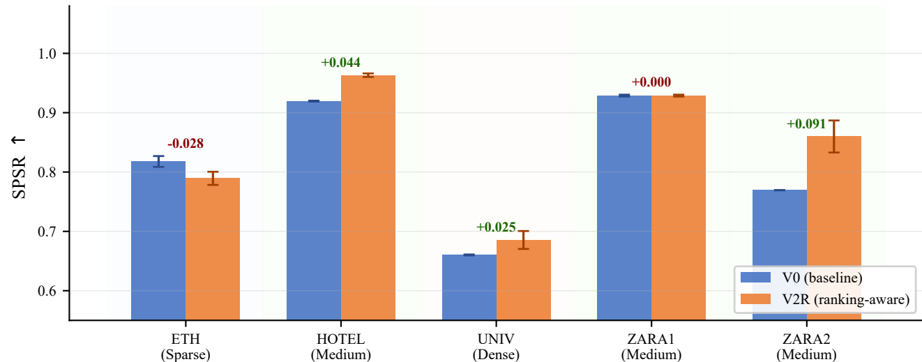
Safe Planning Success Rate by Subset and Density Tier (3-seed mean \pm std; seeds 42, 1, 123)
